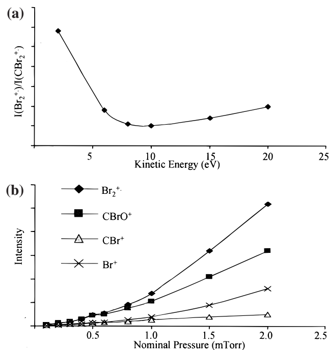
Figure 2. (a) Variation of \text{Br}_2^{+\bullet} intensity with \text{CBr}_2^{+\bullet} collision energy at 0.4 mTorr \text{O}_2 collision gas pressure. (b) Variation of product ion intensities with collision gas pressure at the same collision energy.
