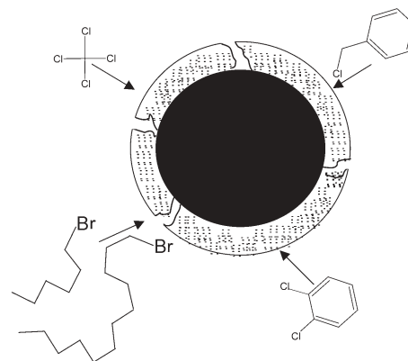
Fig. 6 Schematic representation of a core-shell particle. The shell largely covers the core, but has interconnected channels, which can take molecules such as CCl 4 , CHBr 3 , C 6 H 5 CH 2 Cl, 1-bromohexane and 1-bromododecane into the core where they react with the cores. The alkyl bromides are shown to have gauche defects, as expected in the solution state.
